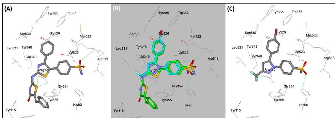
Fig. 6. (A) Docking and binding mode of compound 15b within COX-2 active site (PDB code: 6COX ). (B) The superposition of the docked poses 15b (green) and the co-crystallized S-58701 (cyan) within active site of COX-2. (C) Docking and binding mode of co-crystallized S-58701 into the same COX-2 binding pocket. Hydrogen bonds are represented by dashed green lines. All hydrogens are removed for the purposes of clarity.
