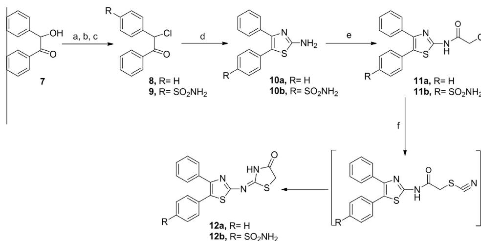
Scheme 1. a Reaction reagents and conditions: (a) SOCl 2 , pyridine, 1 h; (b) chlorosulfonic acid, CH 2 Cl 2 , 0 °C, stirring, overnight; (c) NH 4 OH, THF, rt, 2 h; (d) thiourea, EtOH, reflux, 2 h; (e) ClCH 2 COCl, TEA, CH 2 Cl 2 , rt, 5 h; (f) NH 4 SCN, acetone.
