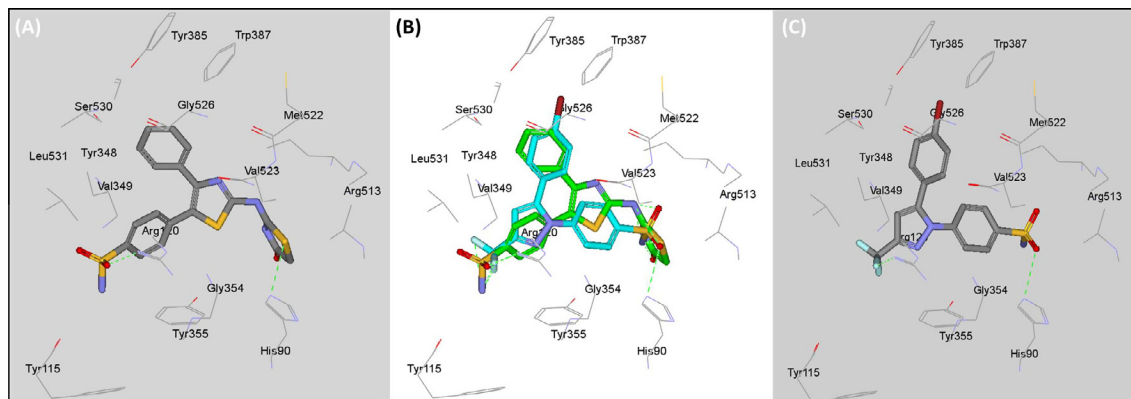
Fig. 7. (A) Docking and binding mode of compound 12b within COX-2 active site (PDB code: 6COX ). (B) The superposition of the docked poses 12b (green) and the co-crystallized S-58701 (cyan) within active site of COX-2. (C) Docking and binding mode of co-crystallized S-58701 into the same COX-2 binding pocket. Hydrogen bonds are represented by dashed green lines. All hydrogens are removed for the purposes of clarity.
